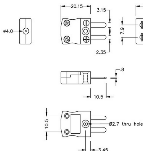
Miniature in-line Plug (dimensions in mm)
